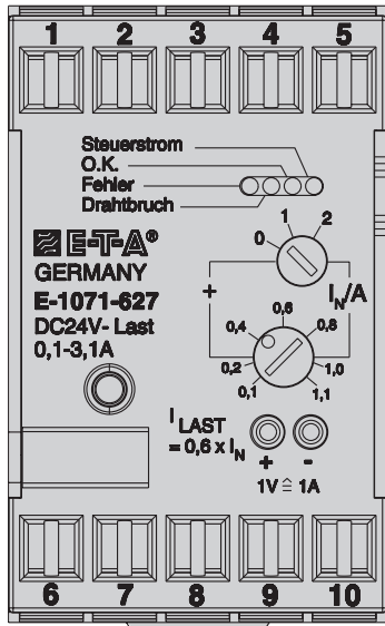
E-1071-627 (0.1 - 3.1 A)
